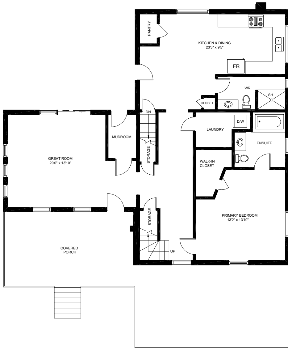
MAIN FLOOR ( 1354 sq.ft.)
